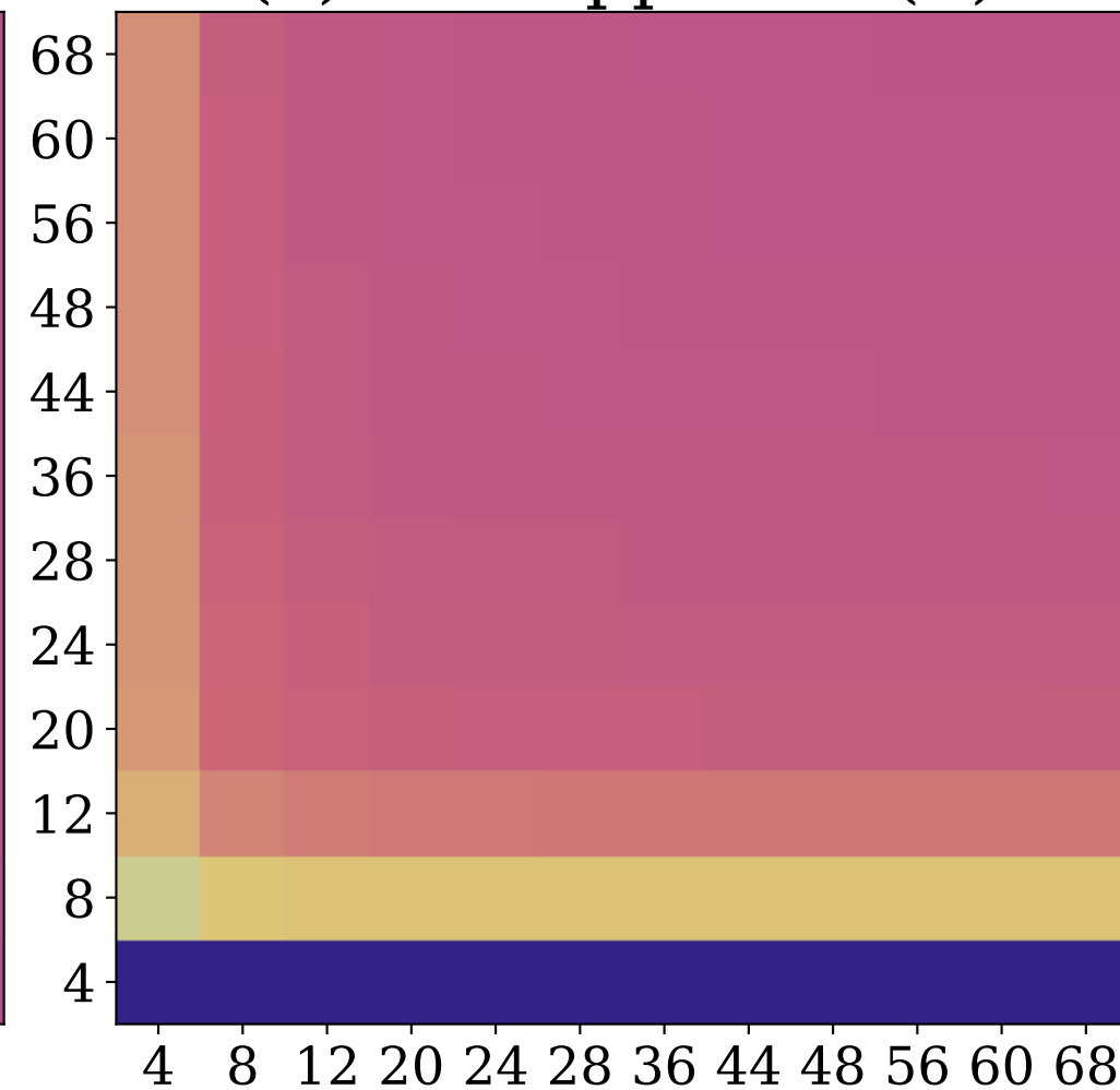
(e) Pair approx. - ( Z )
